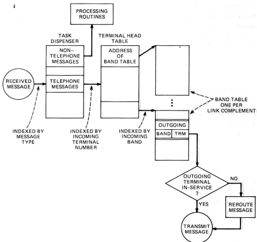
Fig. 5—STP message routing.
